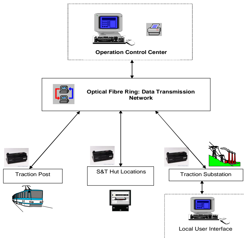
Figure 10.9 - Typical Arrangement of SCADA System for CP- 105 of EDFC
