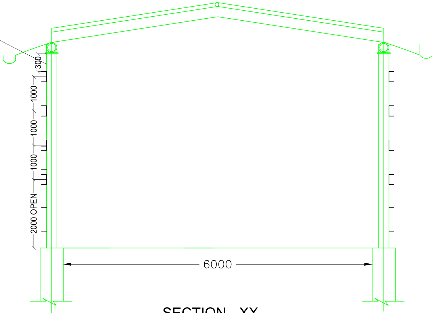
SECTION - XX
