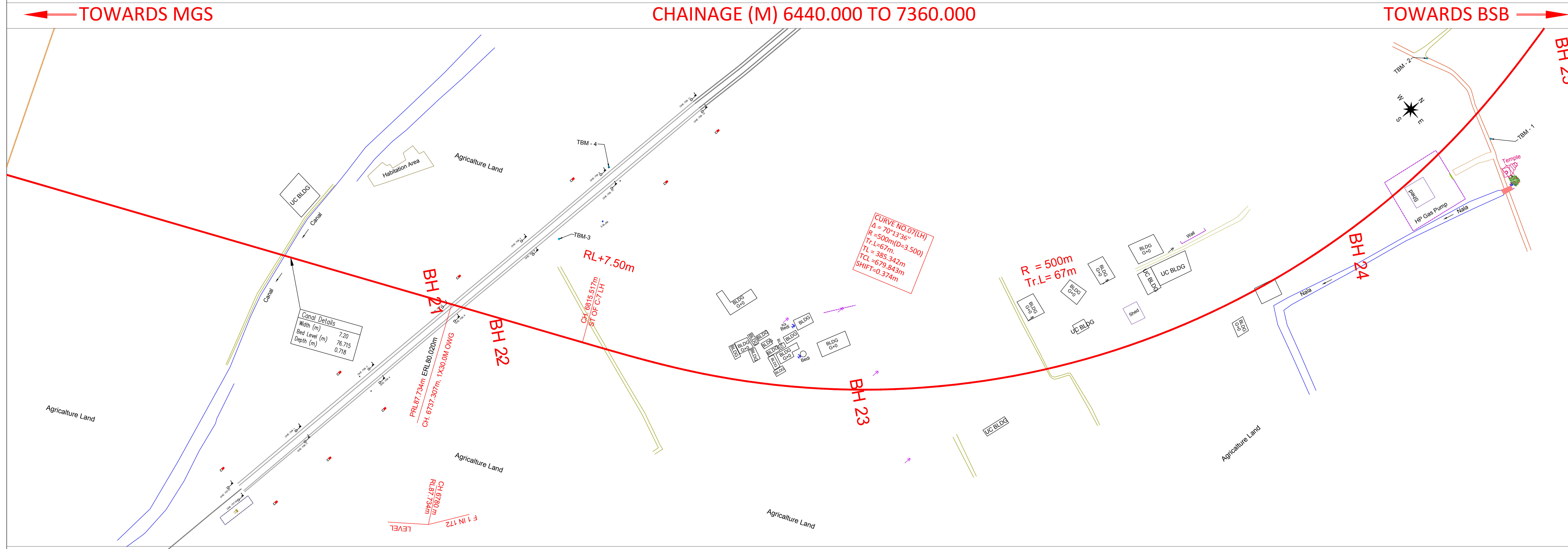
PLAN DRAWING
