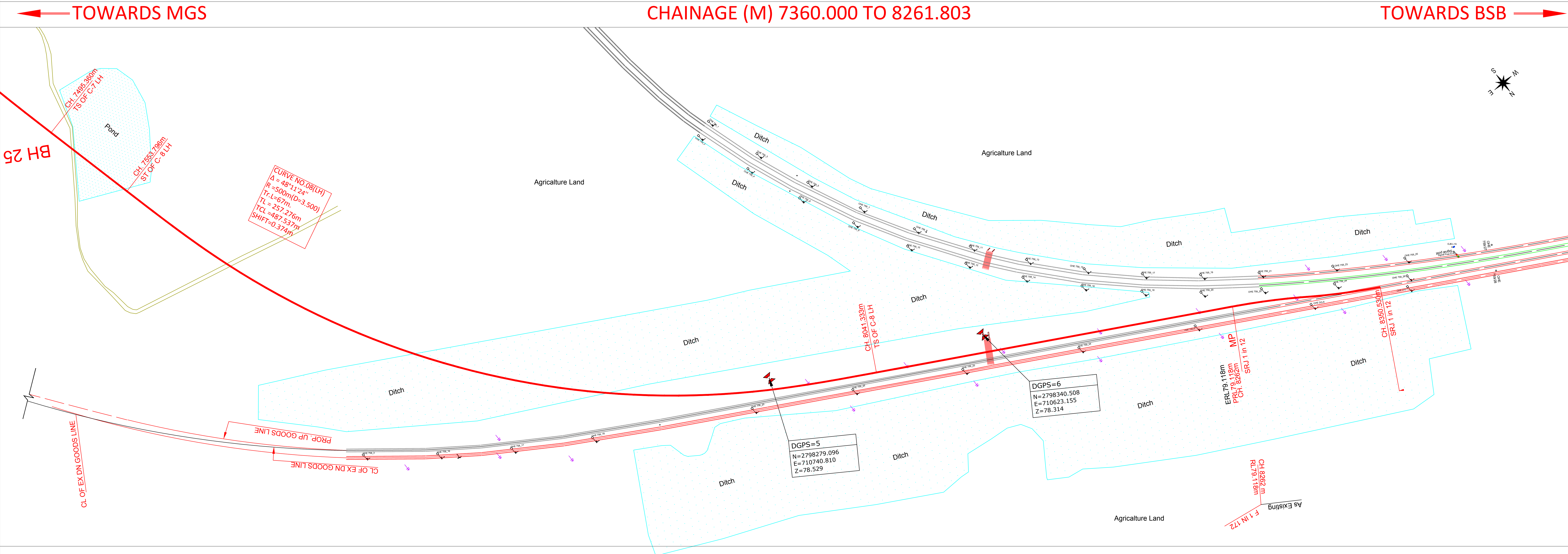
PLAN DRAWING
