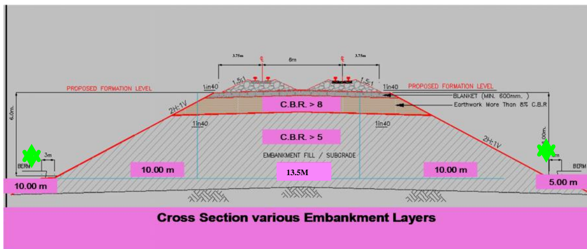
Figure 2-3: Cross Section of the Proposed Freight Corridor
