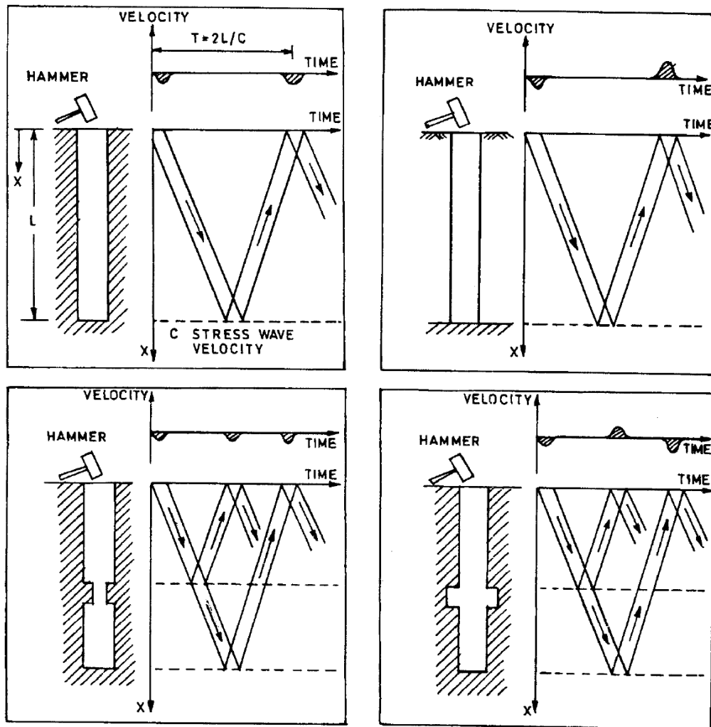
FIG. 1 PATTERN OF STRESS WAVE REFLECTIONS
