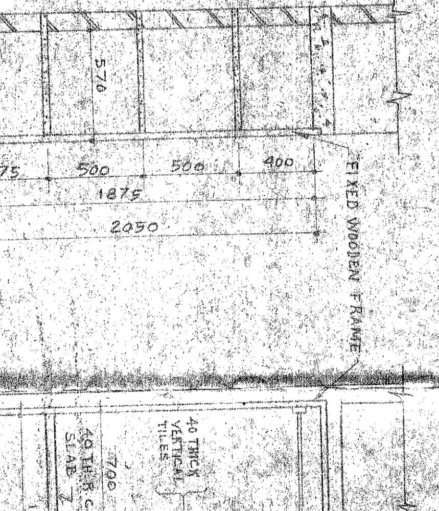
SECTION C-C
